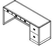
Barrett 72B 72" W x 24" or 30"D x 30"H
